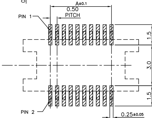
RECOMMENDED PCB LAYOUT GENERAL TOLERANCE ±0.05 WITHOUT BOSS
