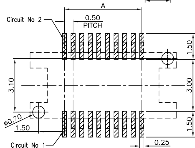
RECOMMENDED PCB LAYOUT GENERAL TOLERANCE ±0.05 WITH BOSS
